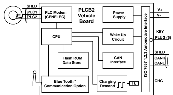
Figure 7 : block diagram of “starter kit”
