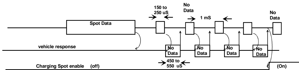
Figure 3: protocol for vehicles without data transfer
