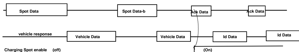
Figure 4: protocol for vehicles with data transfer
